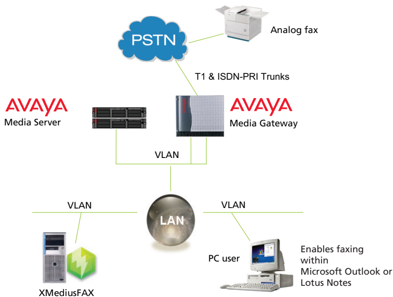
XMediusFAX Seamless Integration with Avaya Communication Manager enables faxing within Microsoft Outlook or Lotus Notes
